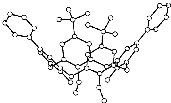
Figure 1. View of compound 13 (hydrogen atoms are omitted for clarity).
